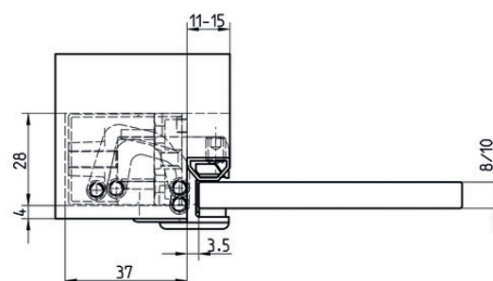
block frame
