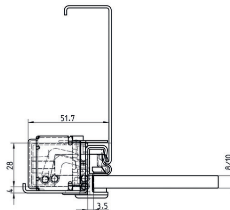
steel frame
